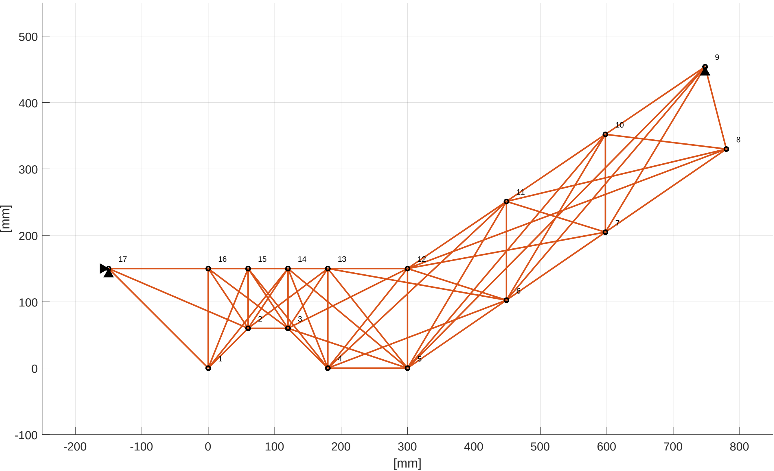
Undeformed structure
